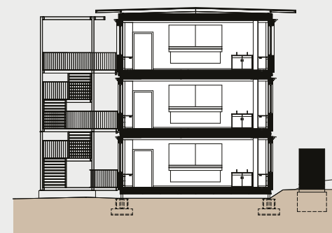
Example cross-section of three-storey building
