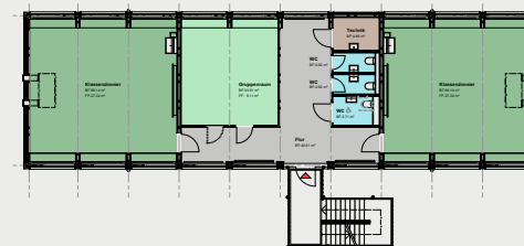
Floor plan for ground floor Ten modules make up one floor
